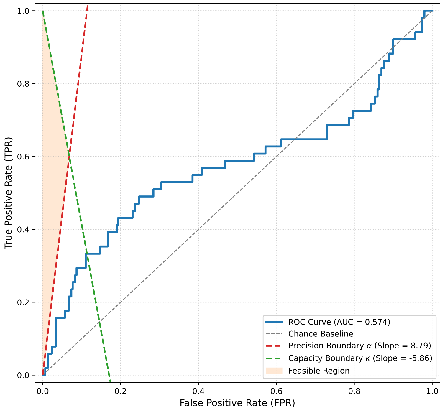
ROC Curve with Dual Slope Bounds ( \alpha & \kappa ): seed_301_101.npy Optimal \theta : 70.7°, c : -1.283
