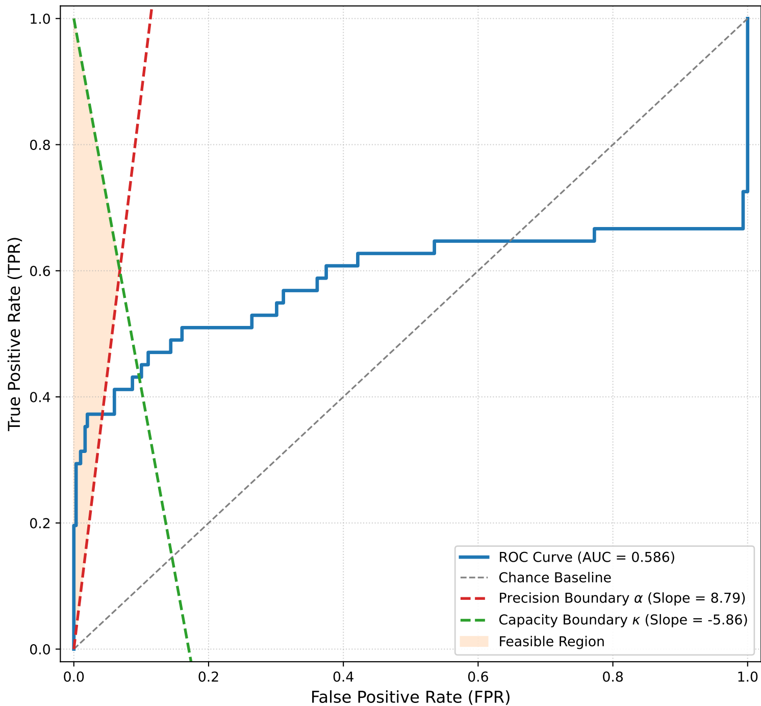
ROC Curve with Dual Slope Bounds ( \alpha & \kappa ): seed_601_201.npy Optimal \theta : 11.4°, c : 0.196
