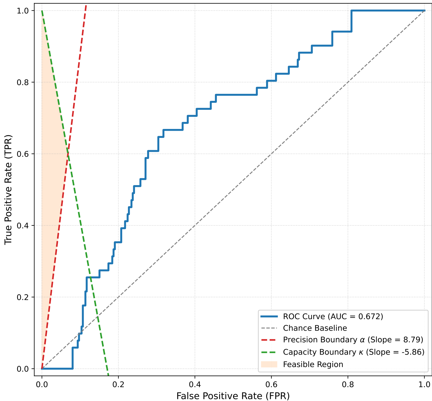
ROC Curve with Dual Slope Bounds ( \alpha & \kappa ): seed_701_501.npy Optimal \theta : 70.7°, c : -1.283
