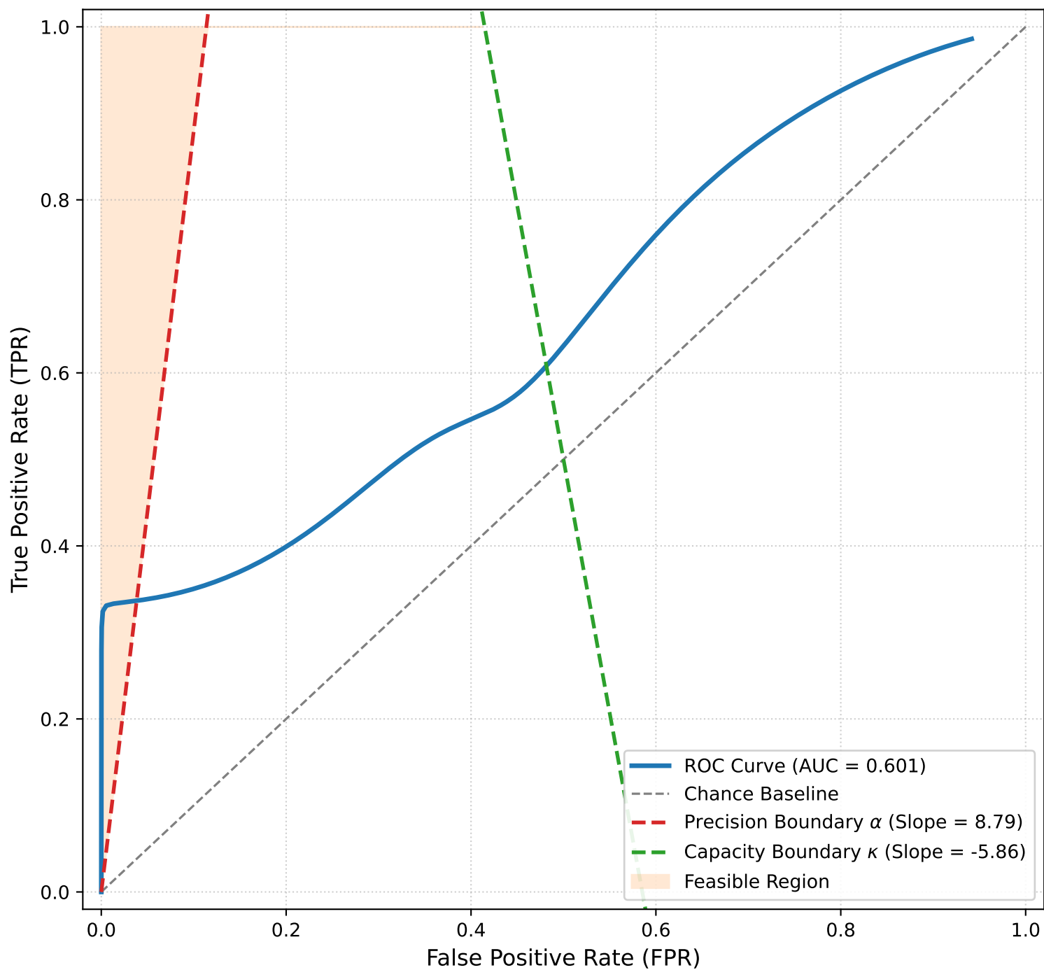
ROC Curve with Dual Slope Bounds ( \alpha & \kappa ): seed_701_501.npy Optimal \theta : 173.9°, c : 1.112
