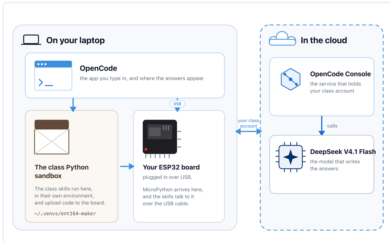
Figure 1. The parts of the system, and where they run. On your laptop: OpenCode, the Python sandbox that runs the class skills and uploads code to the board, and your ESP32 over USB. In the cloud: OpenCode Console and DeepSeek V4.1 Flash, the model that writes the answers.
