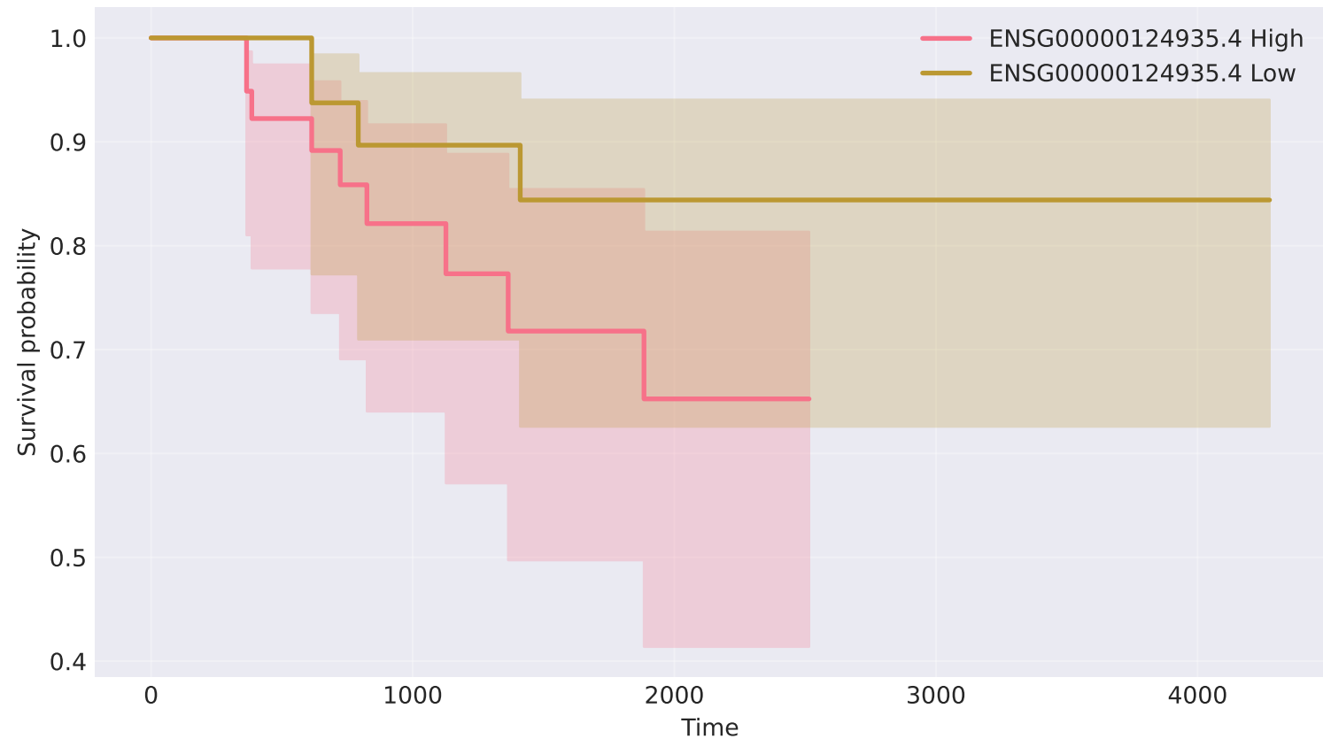
Kaplan-Meier Survival Curve: ENSG00000124935.4
