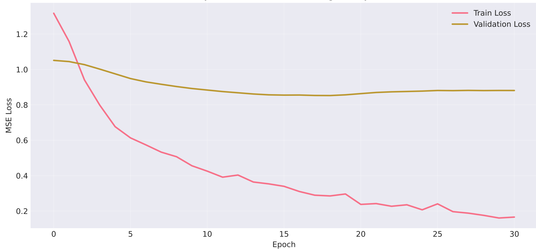
PyTorch Autoencoder Training History
