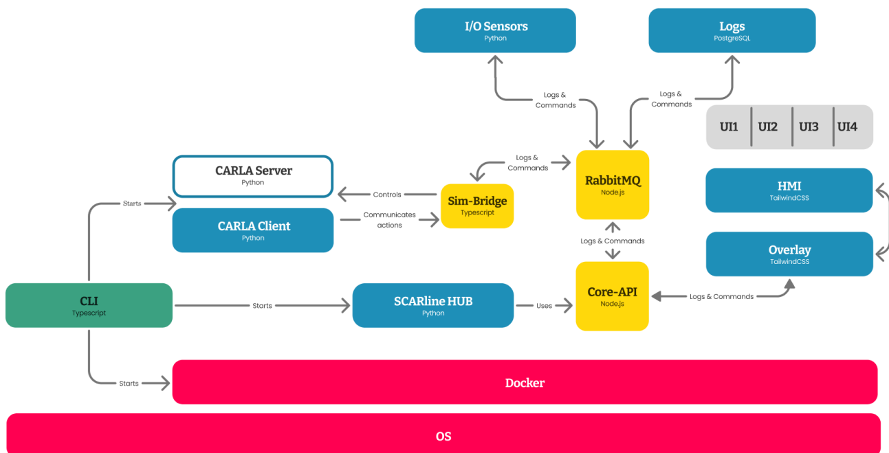
Figure 1: SCARline's full system architecture — This includes the CLI, SCARline Hub, CARLA simulator, Sim-Bridge, RabbitMQ, Core API, I/O sensors, PostgreSQL logging, and the HMI/overlay layer. Docker provides the underlying containerized runtime environment.
