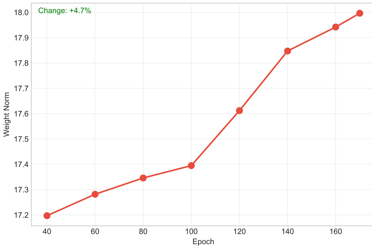
Encoder Self-Attn
