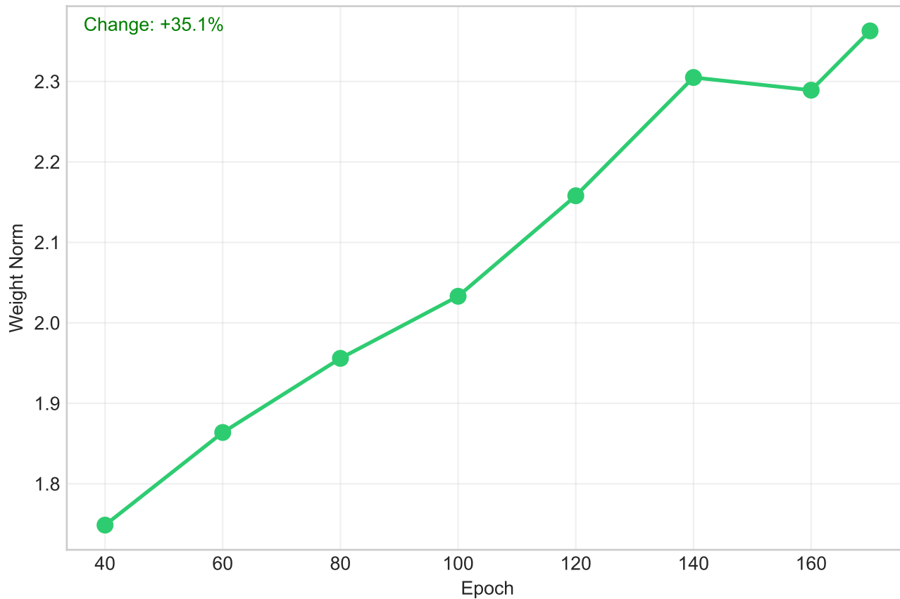
Encoder Self-Attn
