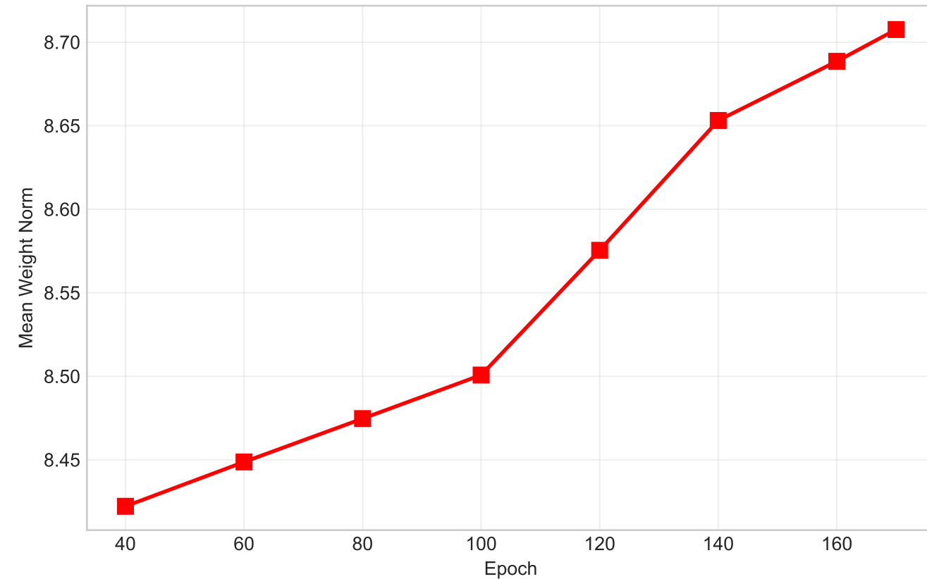
Weight Norm
