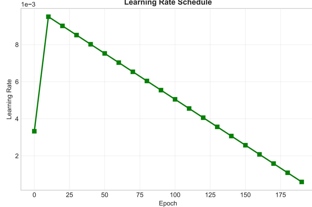
Learning Rate Schedule
