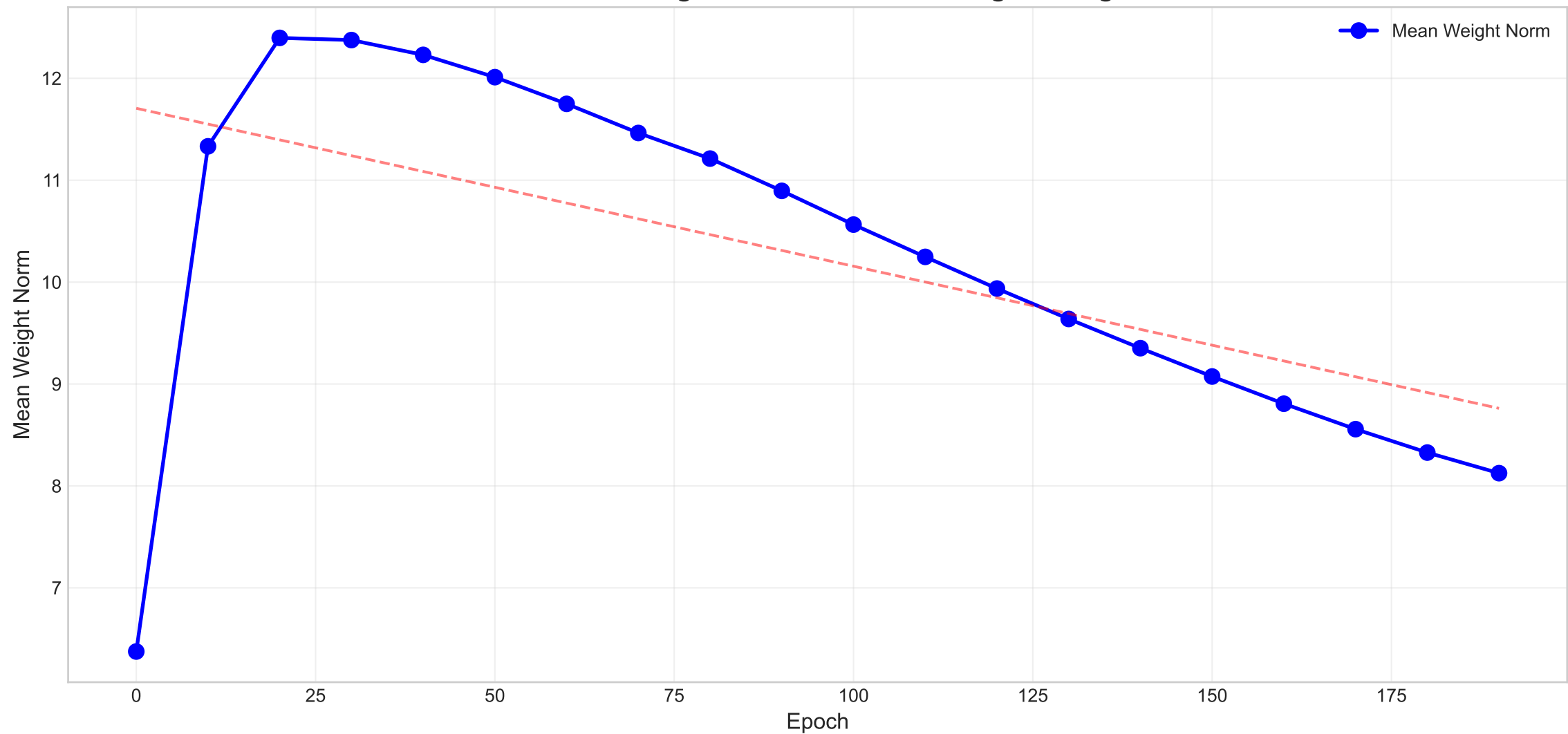
YOLOv8 Weight Norm Evolution During Training
