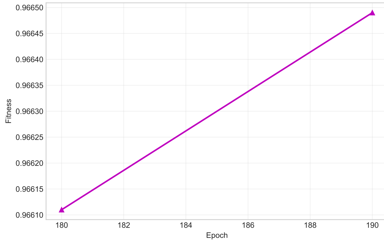
Best Fitness
