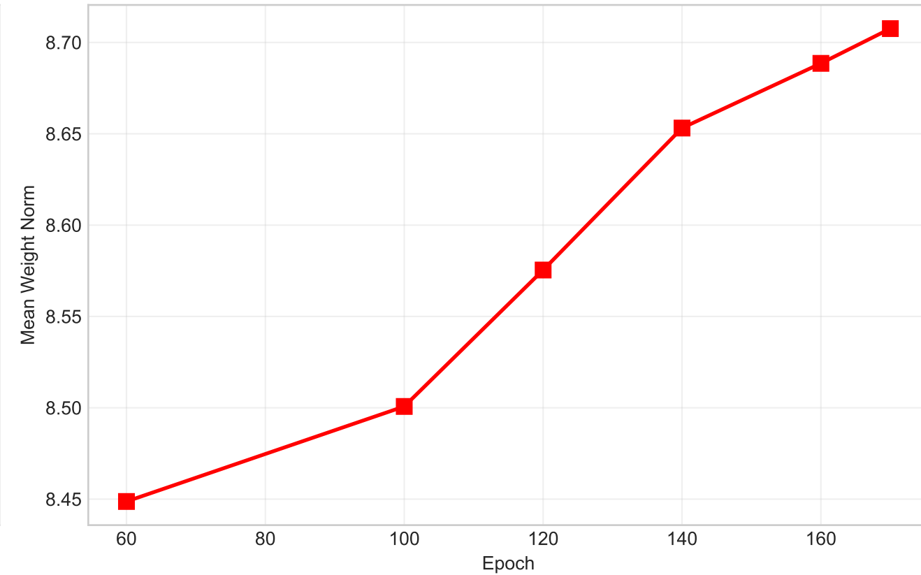
Weight Norm
