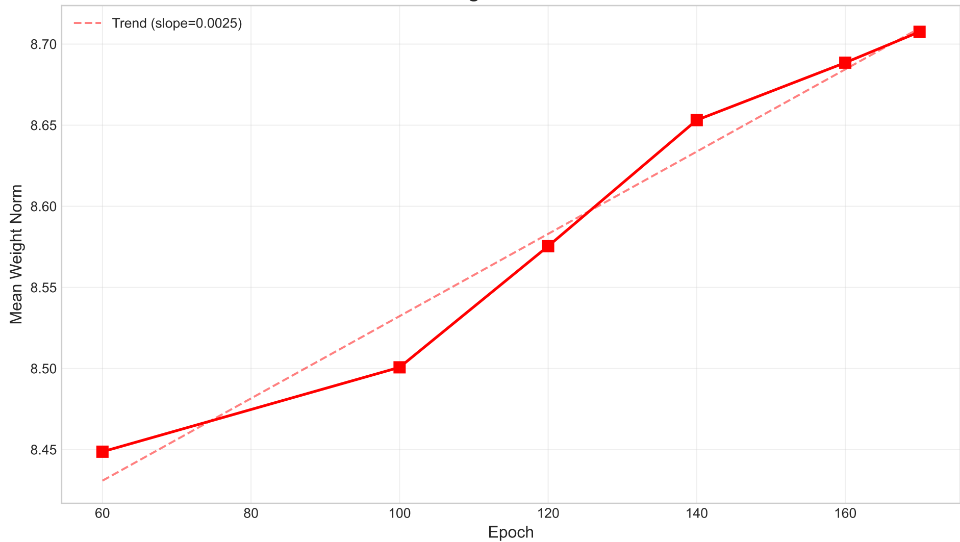
DETR Weight Norm Evolution
