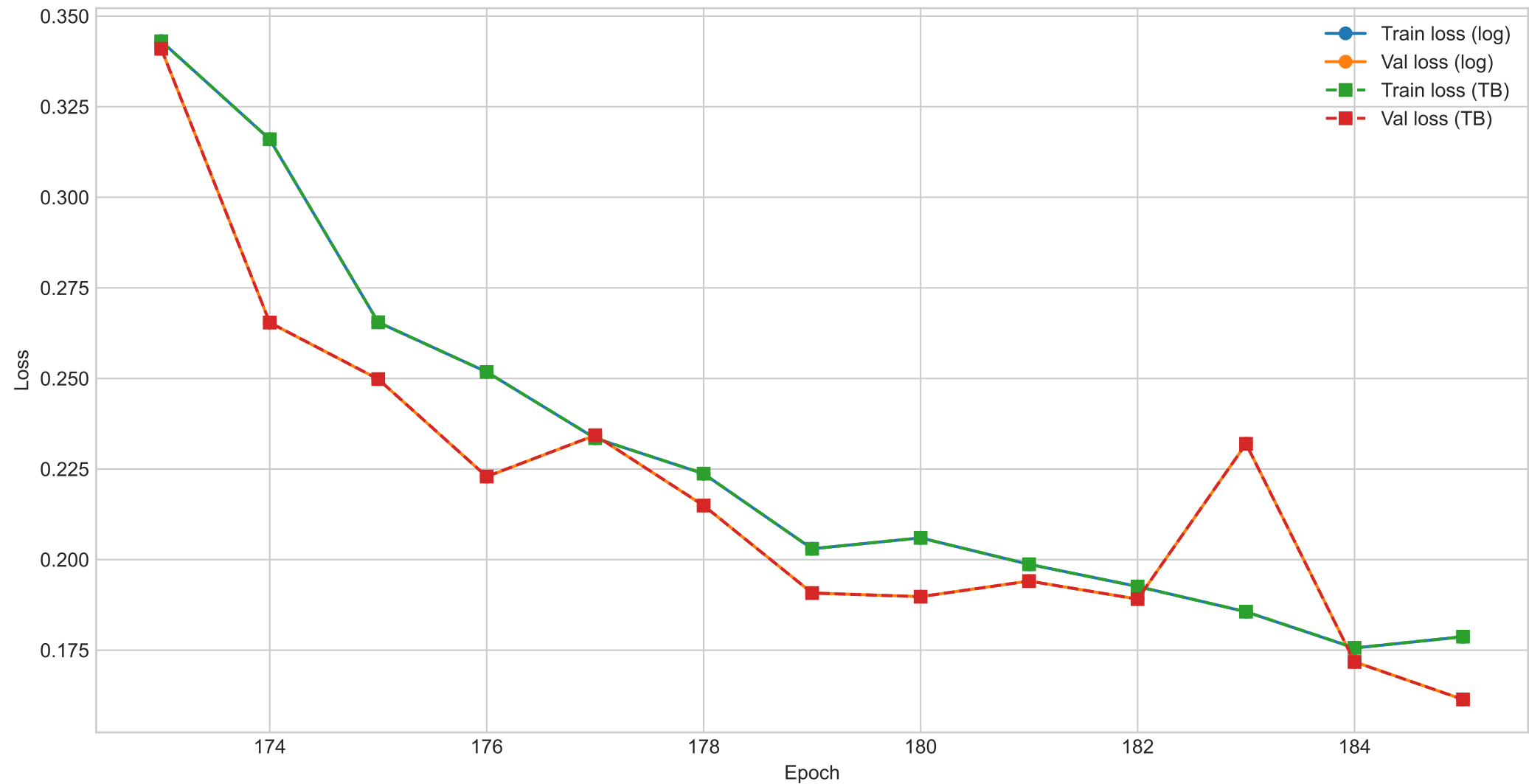
Loss curves
