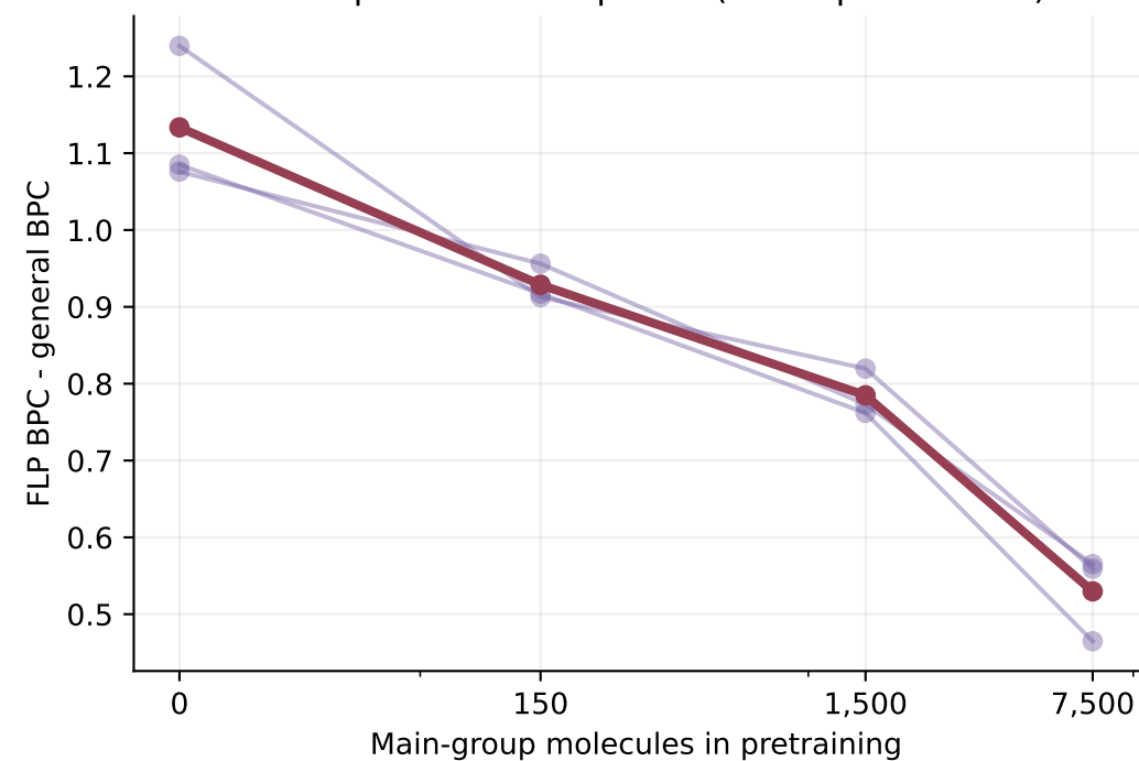
Generation checkpoint sensitivity
