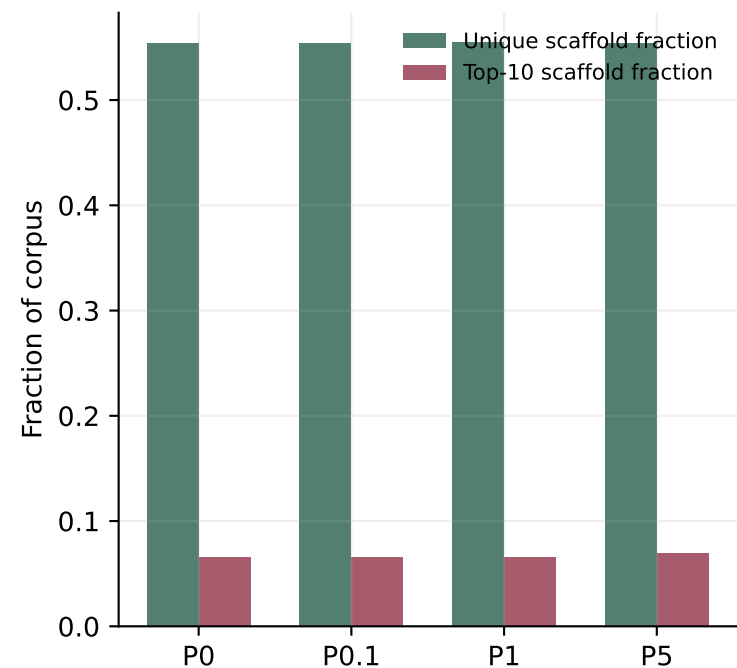
Scaffold distribution
