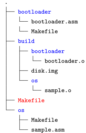
Figure 7.7.4: Top-level Makefile
