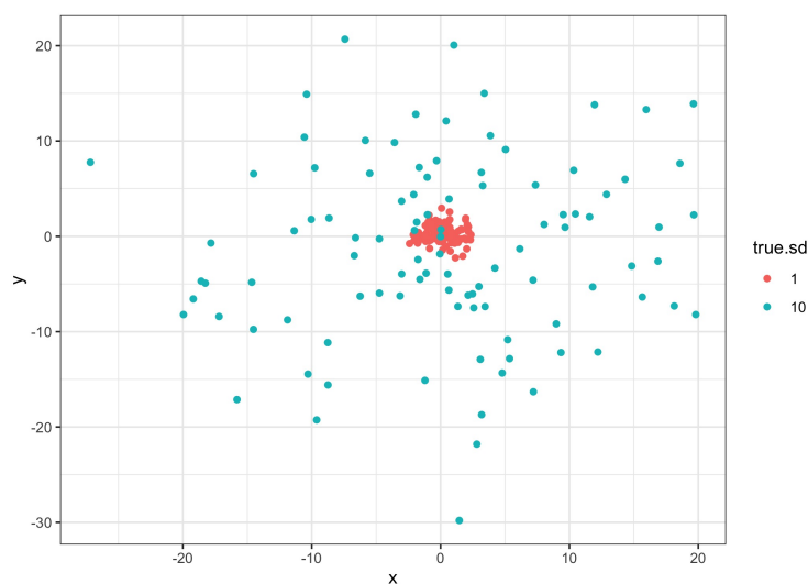
Figure 19.1: Figure 2.1.2. Two samples of 100 numbers drawn from N(0, 1) and N(0, 100) .
