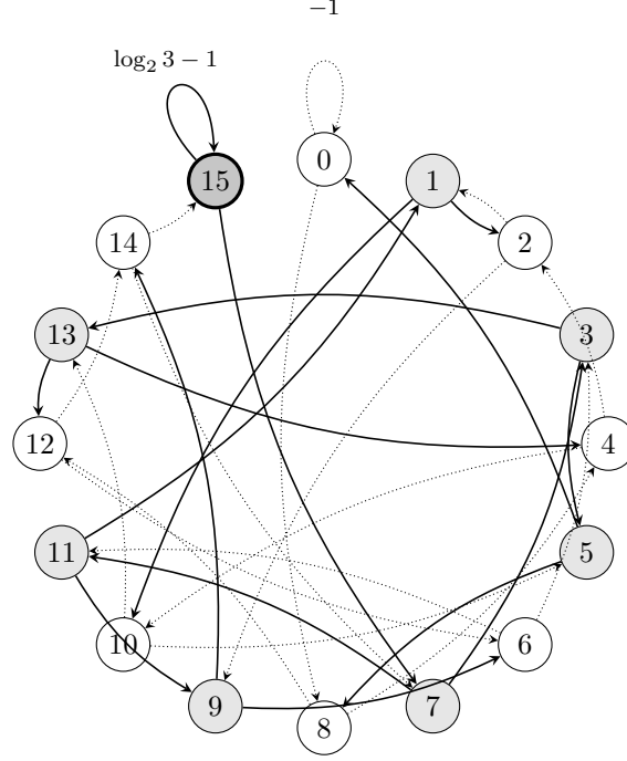
FIGURE 1. The residue graph G_4 on \mathbb{Z}/16\mathbb{Z} (Section 5.3), generated from the laboratory code by paper/make_residue_graph_figure.py (via collatz.invariants.transition_graph_mod2j ). Each residue r has the two successors T(r) \bmod 16 and T(r + 16) \bmod 16 . Solid arcs leave odd residues (shaded) and carry weight \log_2 3 - 1 \approx 0.585 ; dotted arcs leave even residues and carry weight -1 . Exactly two self-loops: at 0 (weight -1 ) and at 15 \equiv -1 \pmod{16} (dark, weight \log_2 3 - 1 > 0 ) — the uncompensable positive-gain loop of Theorem 3.2, returned by Karp’s algorithm as an optimal cycle at every tested level (Section 7.4).
