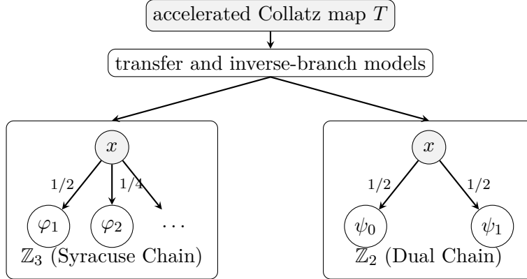
FIGURE 2. Overview of the transfer models associated with the accelerated Collatz map. The Syracuse chain on \mathbb{Z}_3 (left) uses infinitely many branches \varphi_a(x) = (3x+1)2^{-a} with geometric probabilities, encoding the powers of 2 removed after an odd step. The dual inverse-branch chain on \mathbb{Z}_2 (right) uses \psi_0(x) = 2x and \psi_1(x) = \frac{2x-1}{3} with equal probabilities.
