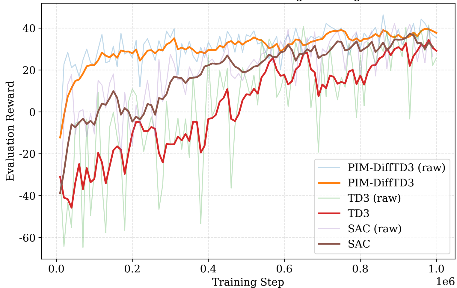
Evaluation Reward During Training
