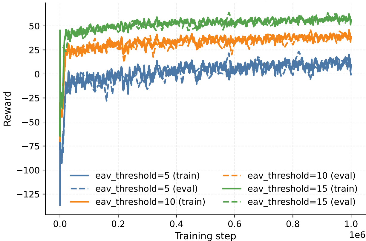
Train / Eval Reward vs Step
