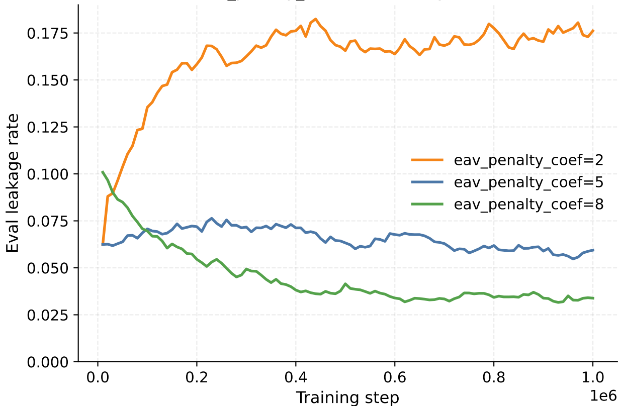
eav_penalty_coef: Eval Leakage Rate
