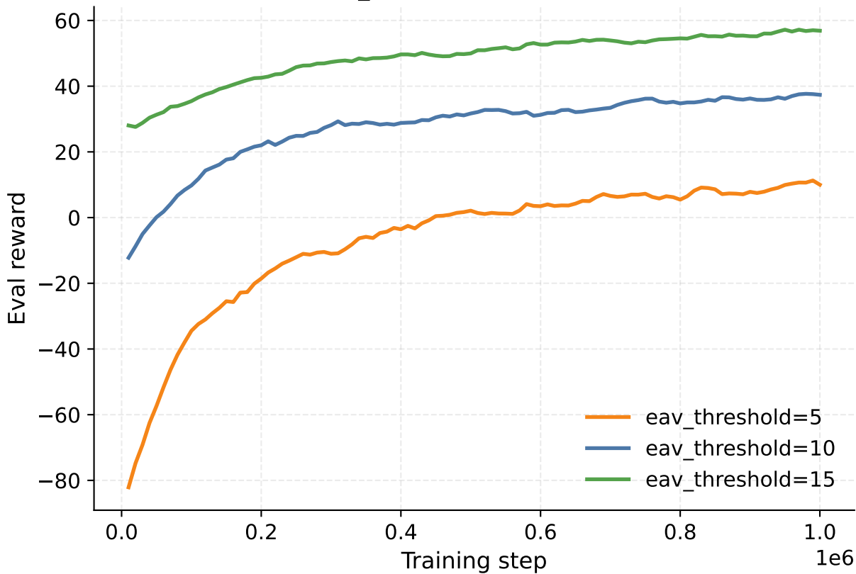
eav_threshold: Eval Reward
