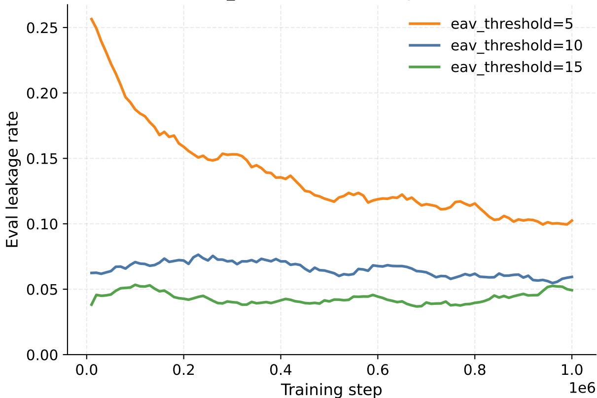
eav_threshold: Eval Leakage Rate
