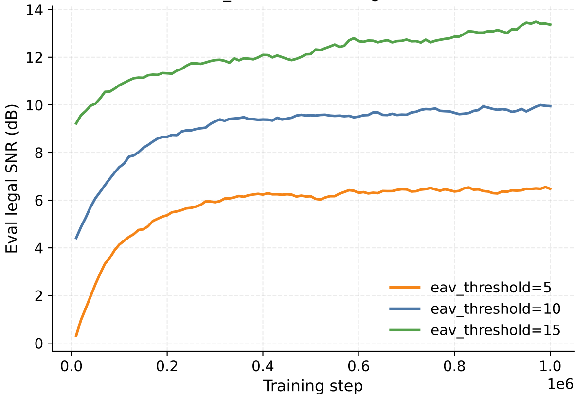
eav_threshold: Eval Legal SNR
