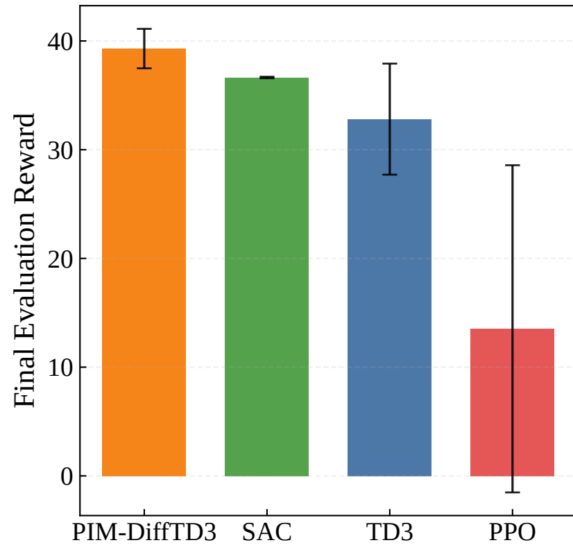
(a) Final Reward
