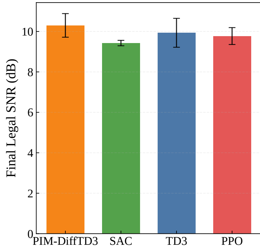
(c) Final Legal SNR
