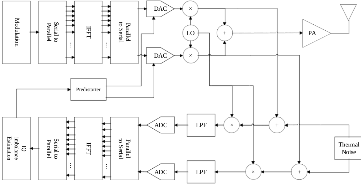
Fig. 1. Transmitter structure with I/Q imbalance predistorter based on RF signal.
