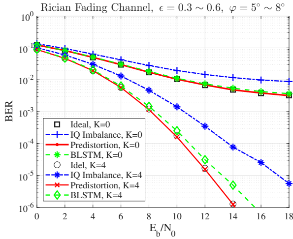
Fig. 4. BER performance with and without I/Q imbalance predistortion over a Rician fading channel
