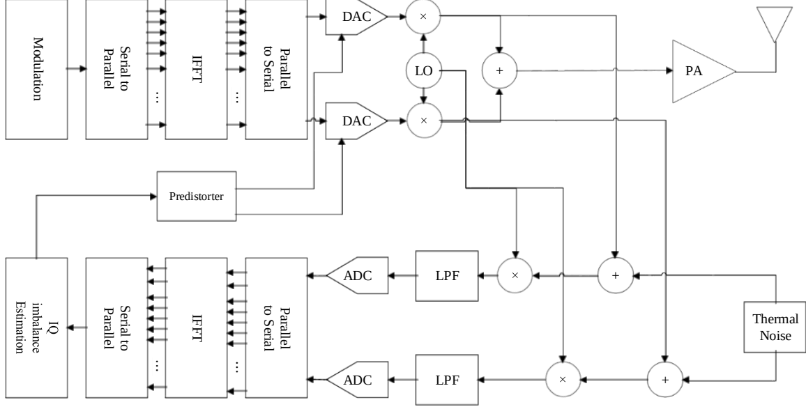
Fig. 1. Transmitter structure with I/Q imbalance predistorter based on RF signal.
