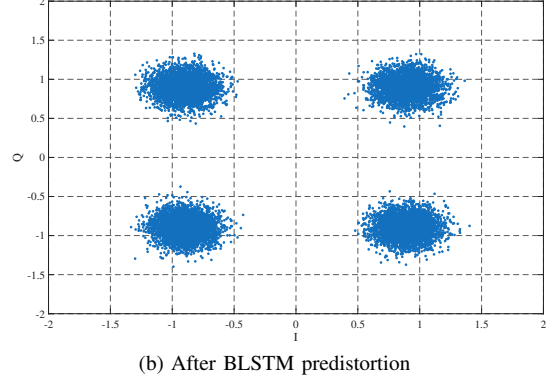
Fig. 3. Signal constellations in AWGN at E_b/N_0 = 15 dB.
