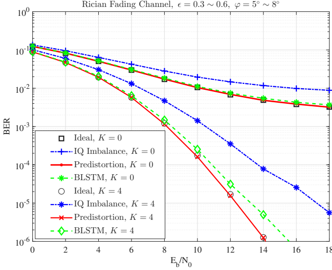
Fig. 5. BER performance with and without I/Q imbalance predistortion in Rician fading channel
