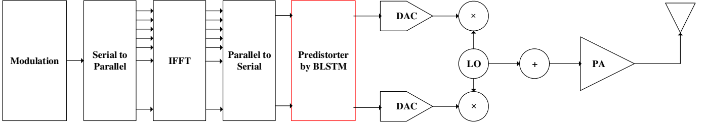
Fig. 3. The example of transmitter structure with I/Q imbalance predistorter by BLSTM
