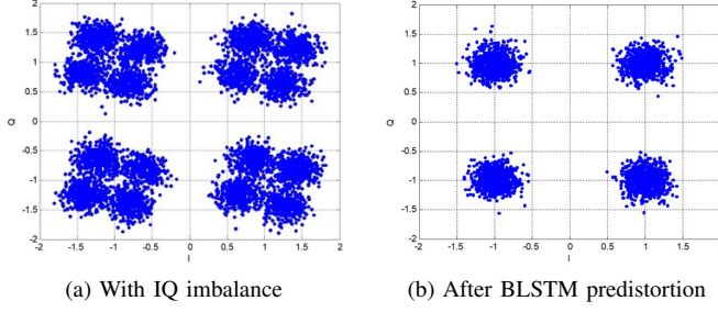
Fig. 4. Signal constellations in AWGN at E_b/N_0 = 15 dB.
