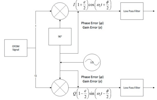
Fig. 1. I/Q imbalance of the local oscillator
