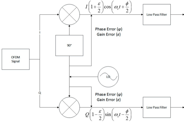
Fig. 1. I/Q imbalance of the local oscillator
