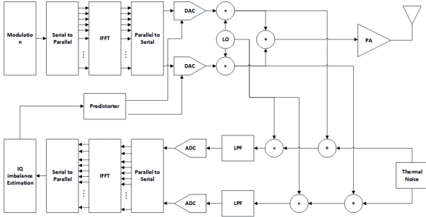
Fig. 2. Transmitter structure with I/Q imbalance predistorter based on RF signal.
