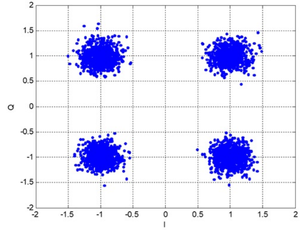
Fig. 5. Signal constellation in an AWGN channel after I/Q imbalance compensation
