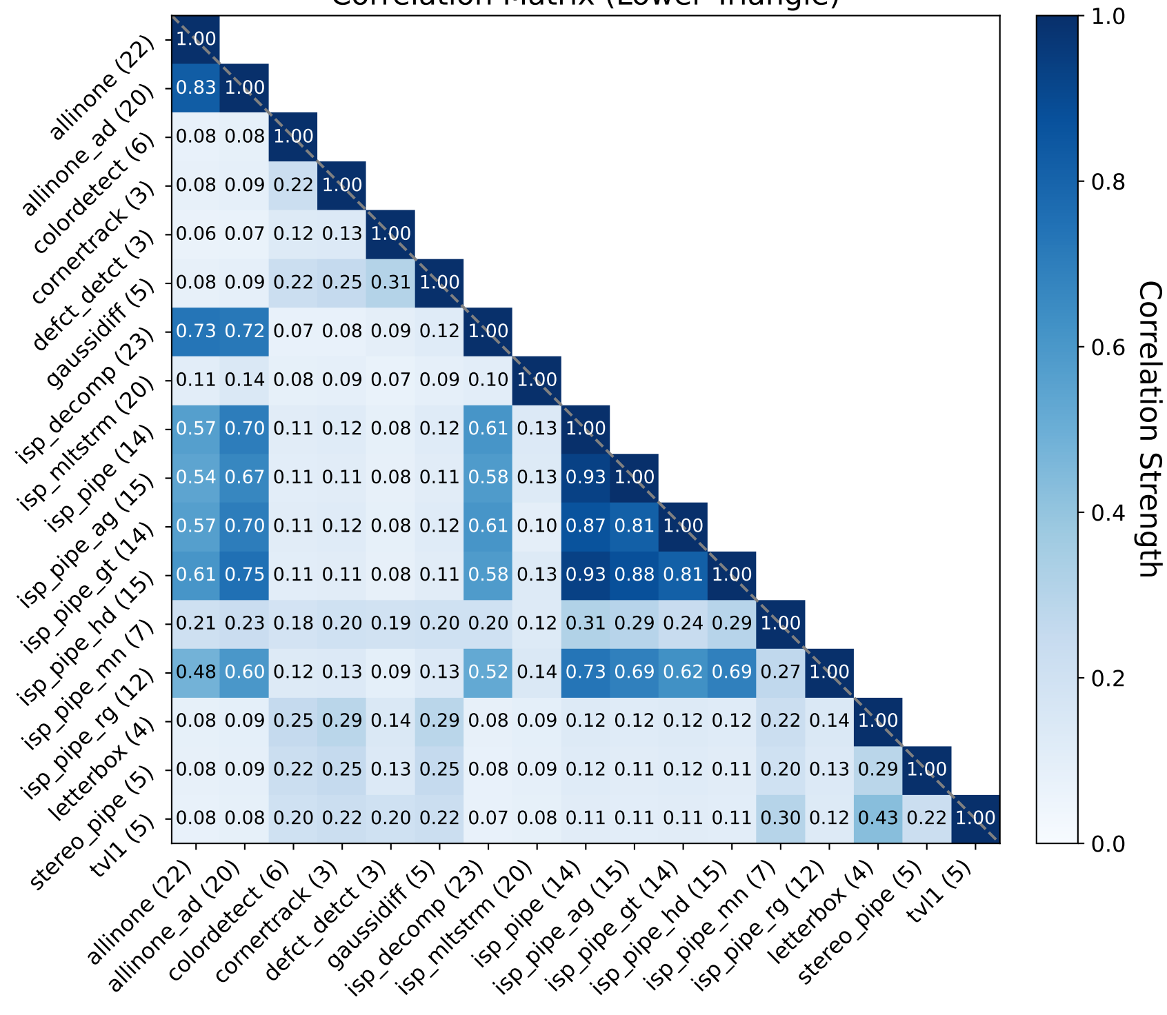
Correlation Matrix (Lower Triangle)
