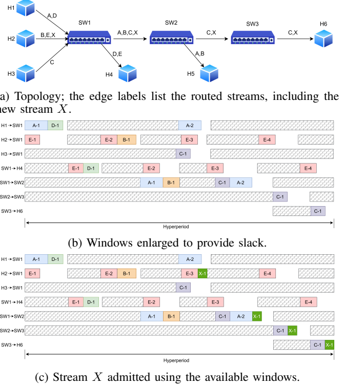
Fig. 3: WPEx example: (a) the topology; (b) enlarged TAS windows provide slack; (c) a new stream X uses the available windows without changing the GCL.
