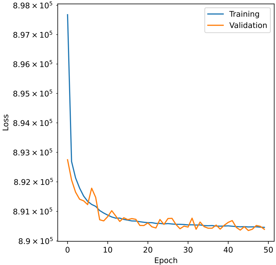
Loss
