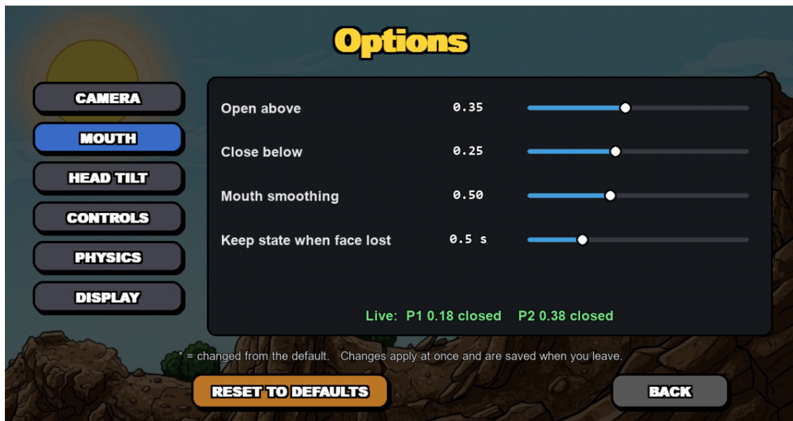
The Mouth tab. The green line shows each player's live mouth score, so the thresholds can be set while watching it. A gold * marks a changed value.
