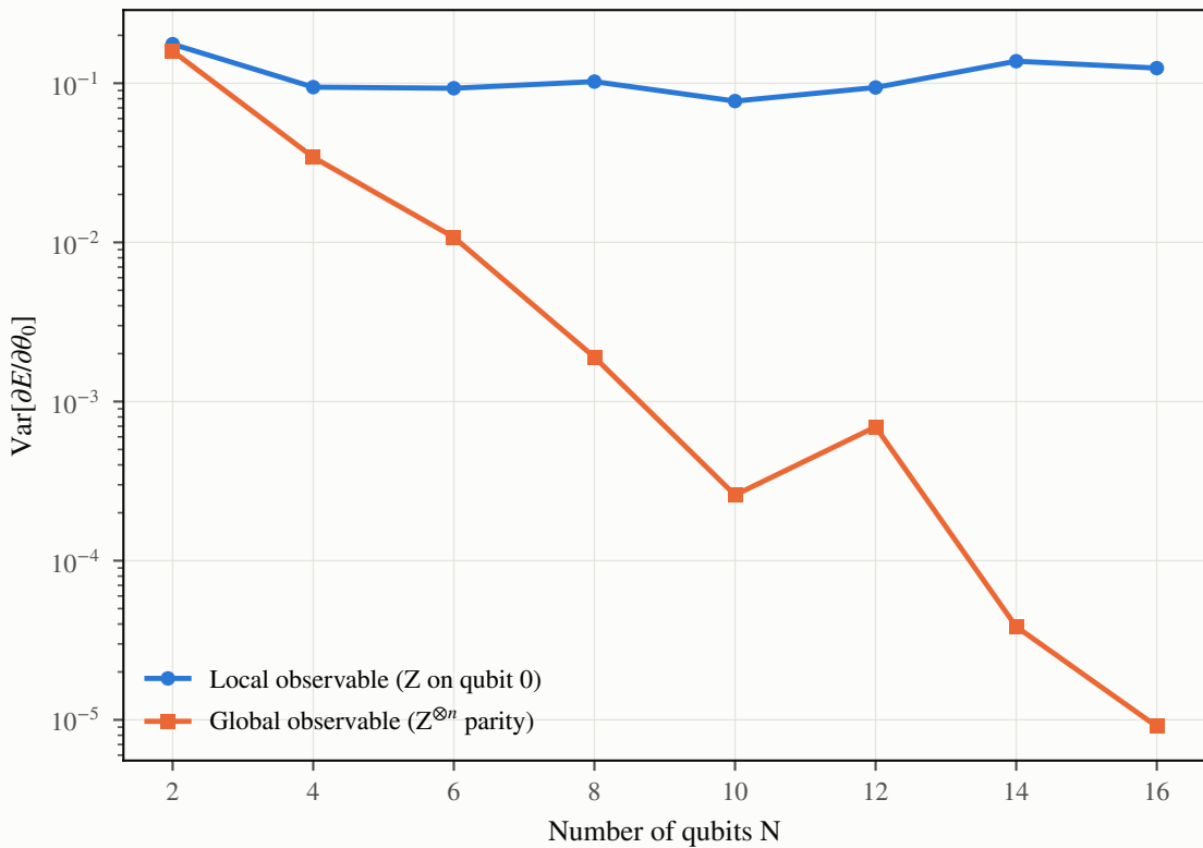
Barren plateaus: local vs. global cost function (EfficientSU2, reps=3)
