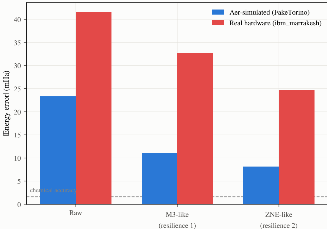
Simulation vs. real hardware: H2/EfficientSU2 on a Heron-class device
