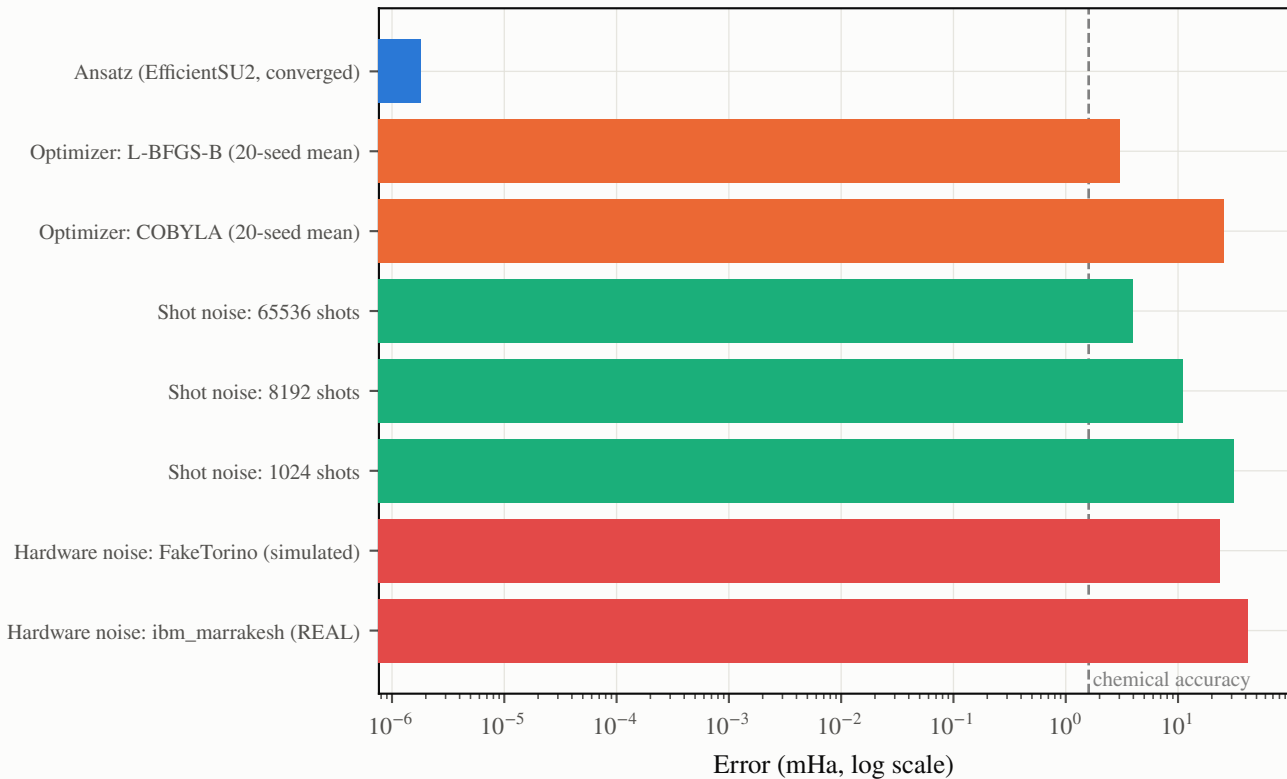
H2/STO-3G error budget: independently-measured term magnitudes
