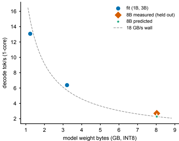
Two-pillar: micro→end-to-end 8B pred 2.28 vs meas 2.70 (16% err)
