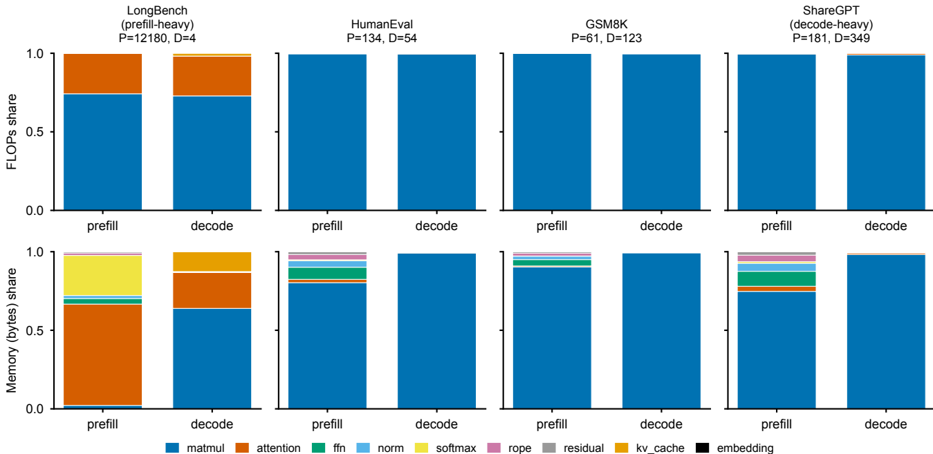
Op-category composition — Qwen2.5-7B (matmul dominates compute & memory; attention rises in long-context prefill)
