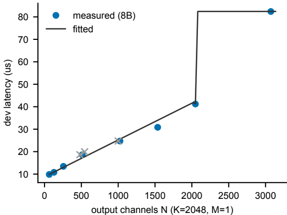
P1 CIM channel-64 staircase
