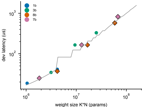
P2 CIM decode GEMV fit (diamond=held-out 8B/Qwen)
