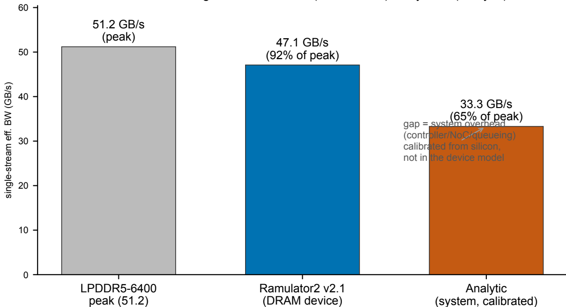
LPDDR5-6400 single-stream: device (Ramulator2) vs system (analytic)
