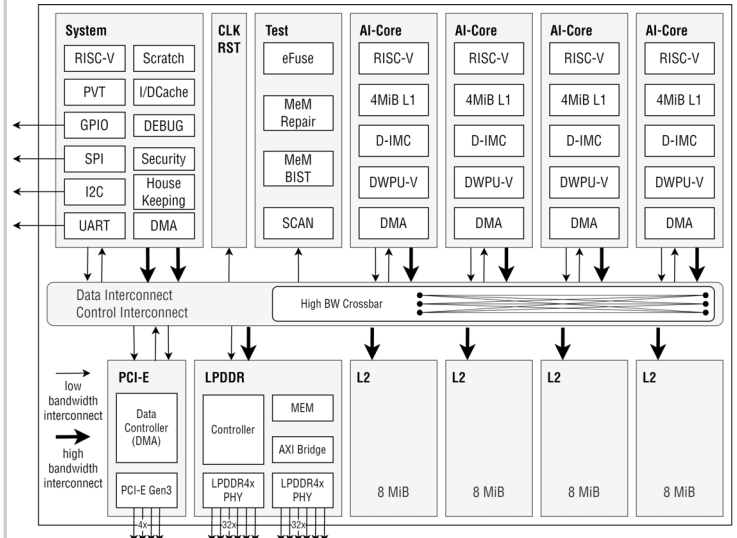
Figure 11.3.2: Metis AIPU SoC architecture.
