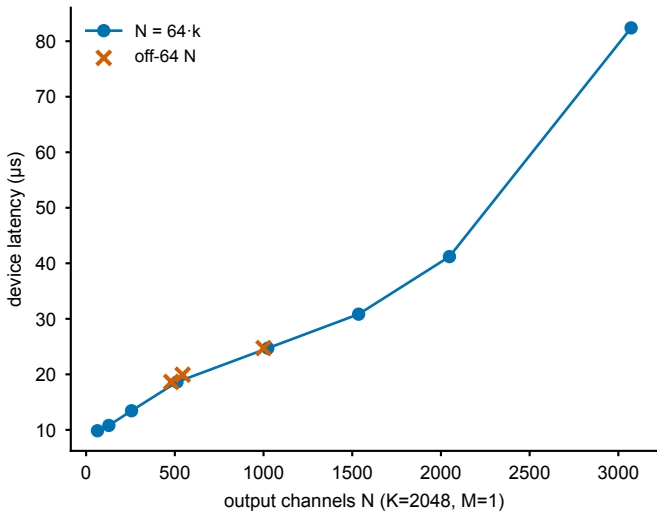
CIM channel-tile (64) staircase (A1d.2)
