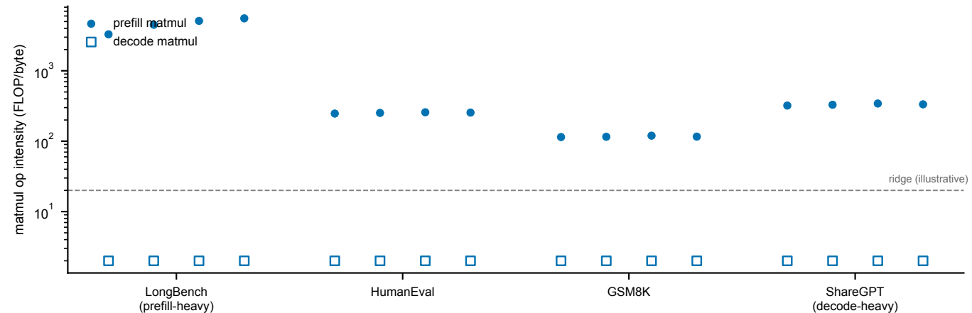
matmul: prefill (compute-bound, high intensity) collapses to decode GEMV (memory-bound, ~1) — 4 models
