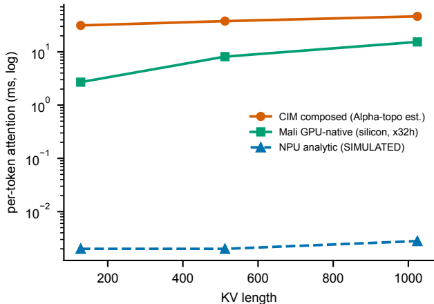
N2 attention offload — Mali silicon / CIM Alpha-est (solid) vs NPU (dashed, sim)
